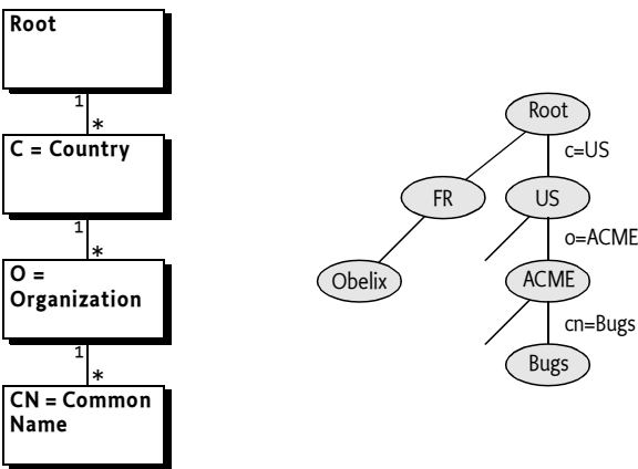
Figure 2.7 Country, Company, Person based name space.
