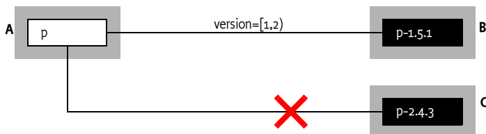
Figure 3.13 Version Constrained
