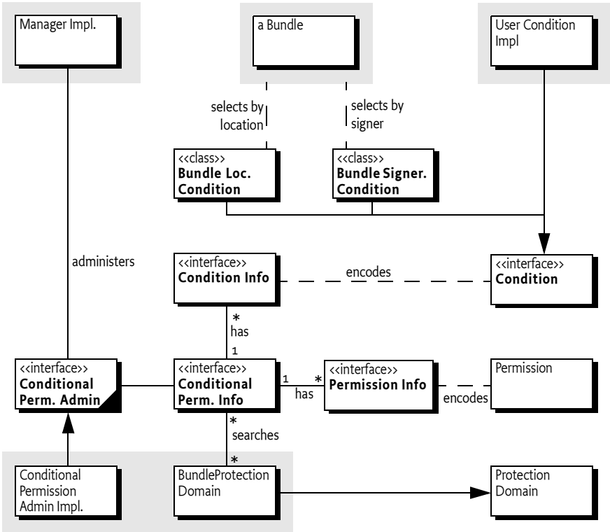
Figure 9.34 org.osgi.service.condpermadmin package
