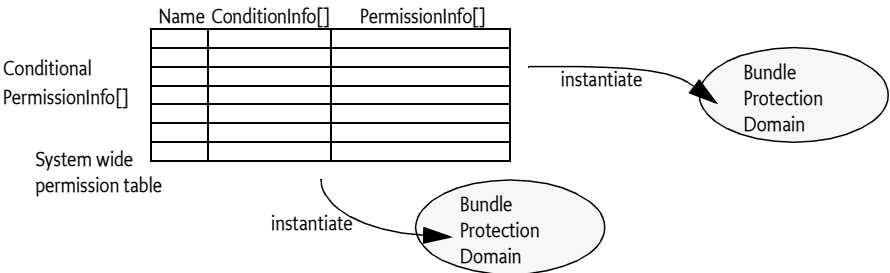
Figure 9.40 Instantiation of the permission table
