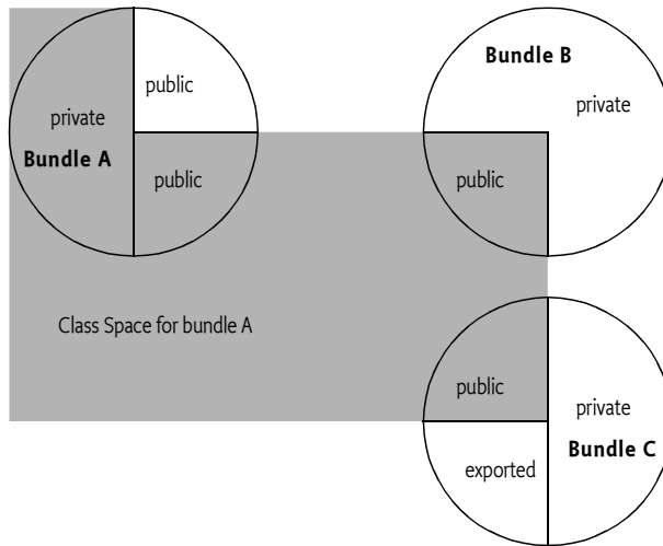
Class Space
