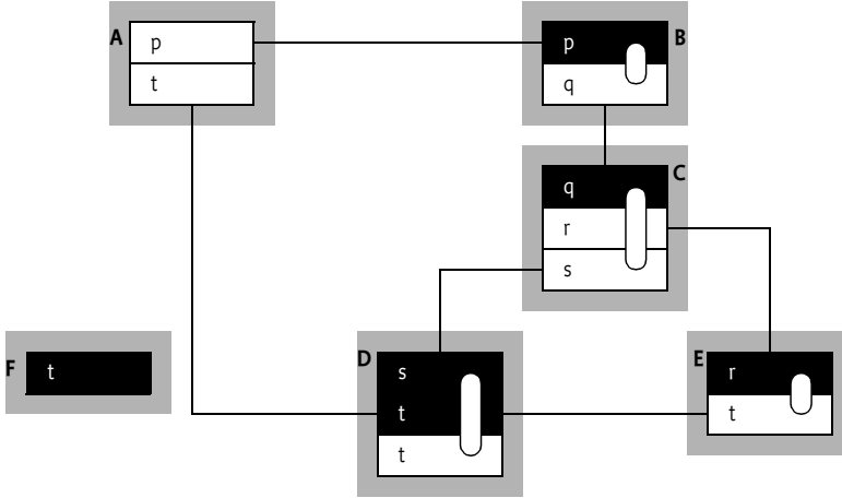
Figure 3.16 Implied Packages
