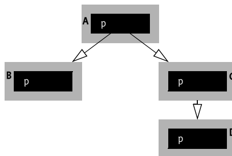
Figure 3.19 Depth First search with Require Bundle
