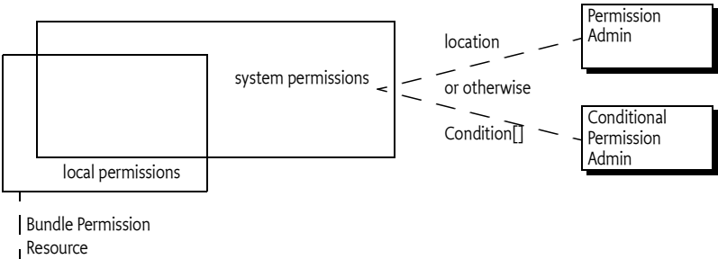
Figure 9.39 System, Local and Security permissions
